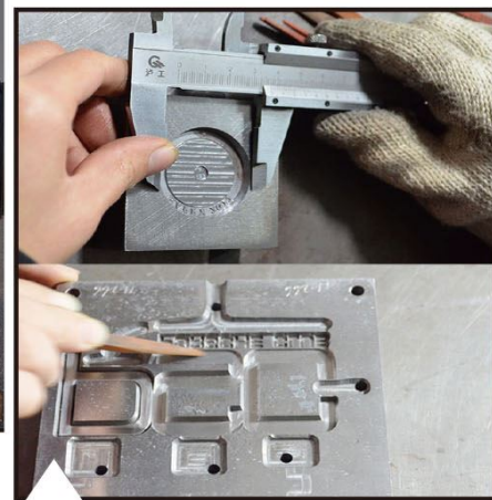
03 Smooth/polish the mould
